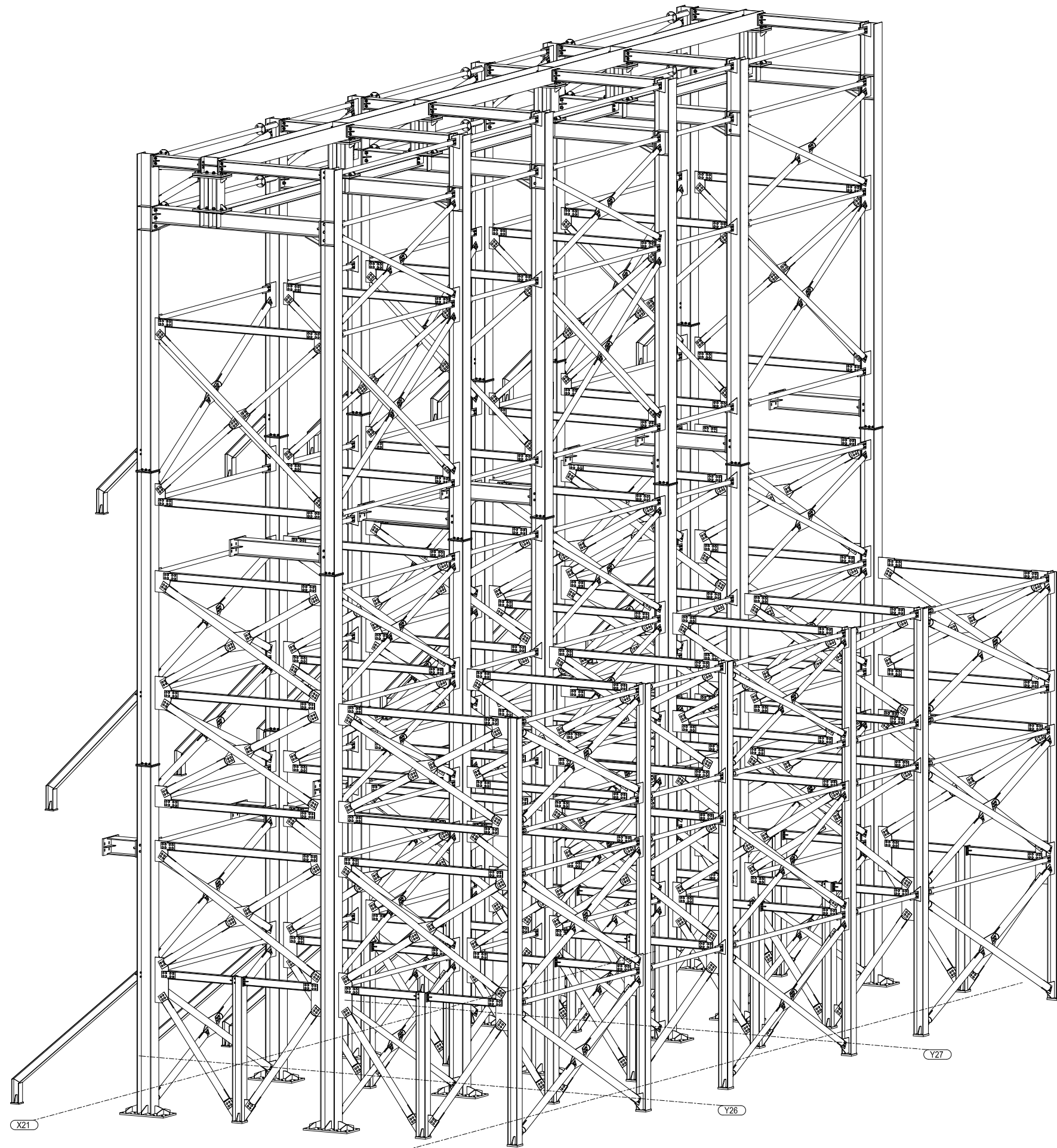
ISOMETRIC VIEW
